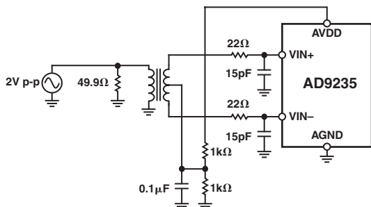
Figure 9. Differential Transformer-Coupled Configuration
