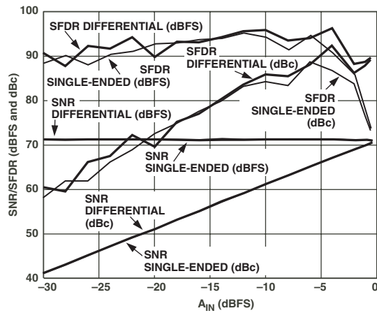
TPC 9. AD9235-20: Single Tone SNR/SFDR vs. A_{IN} with f_{IN} = Nyquist (10 MHz)
