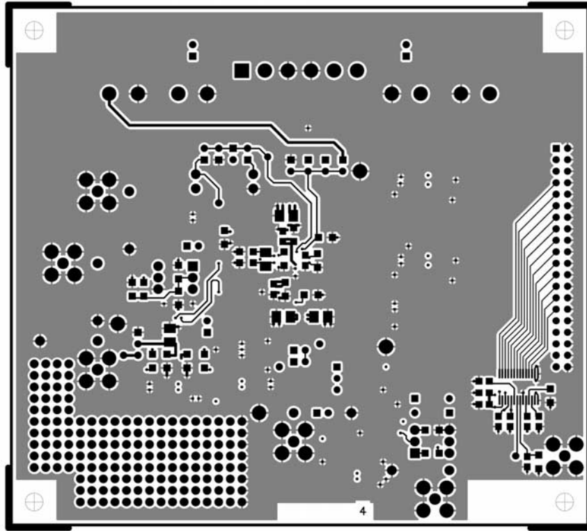
Figure 22. TSSOP Evaluation Board Layout, Secondary Side
