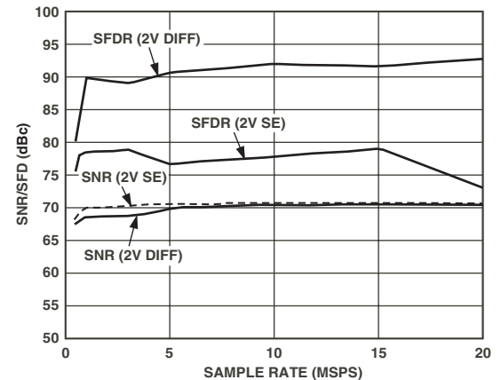
TPC 6. AD9235-20: Single Tone SNR/SFDR vs. f_{\text{CLK}} with f_{\text{IN}} = \text{Nyquist} (10 MHz)
