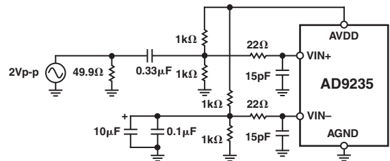
Figure 10. Single-Ended Input Configuration
