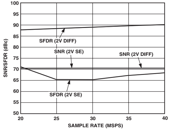
TPC 5. AD9235-40: Single Tone SNR/SFDR vs. f_{\text{CLK}} with f_{\text{IN}} = \text{Nyquist} (20 MHz)
