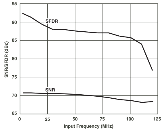
TPC 11. AD9235-40: SNR/SFDR vs. f_{IN}
