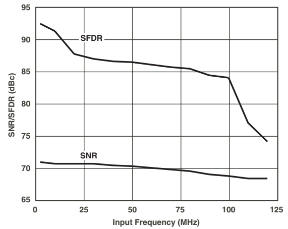
TPC 12. AD9235-20: SNR/SFDR vs. f_{IN}
