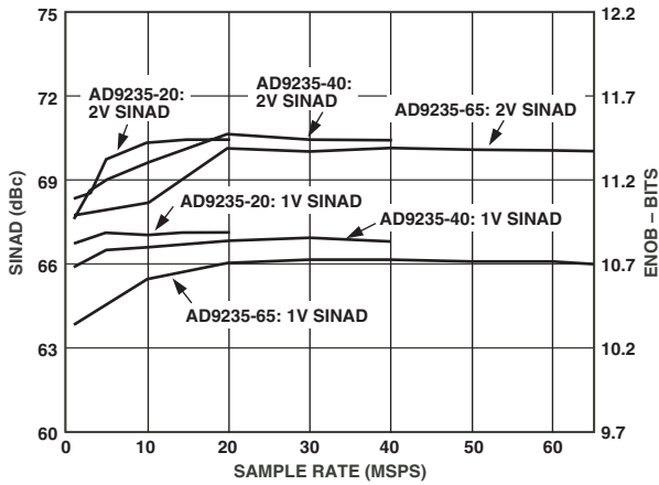
TPC 19. SINAD vs. f_{CLK} with f_{IN} = Nyquist
