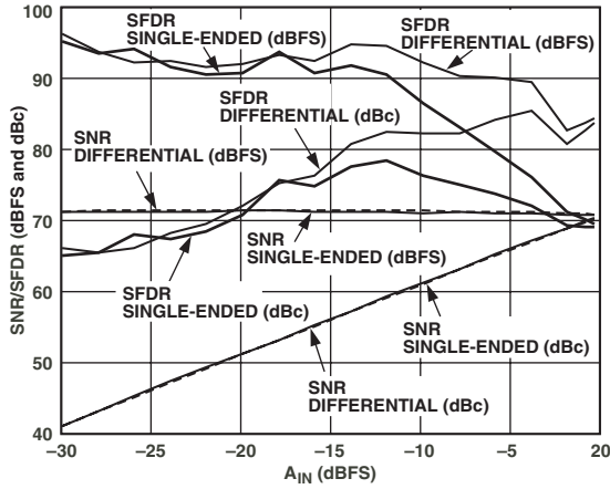
TPC 7. AD9235-65: Single Tone SNR/SFDR vs. A_{IN} with f_{IN} = Nyquist (32.5 MHz)
