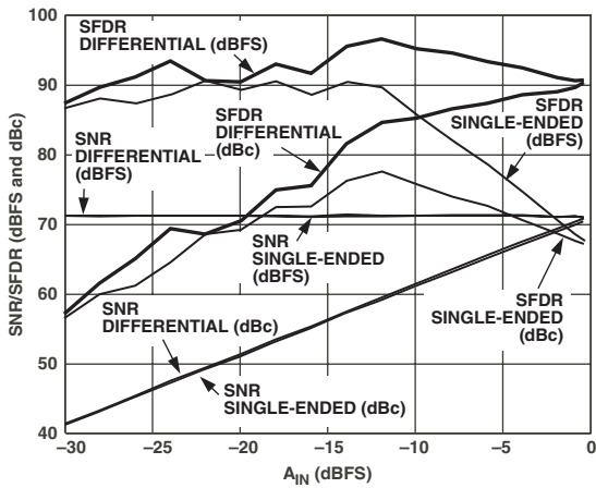
TPC 8. AD9235-40: Single Tone SNR/SFDR vs. A_{IN} with f_{IN} = Nyquist (20 MHz)
