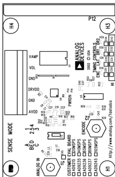
Figure 34. LFCSP Evaluation Board Layout, Primary Silkscreen
