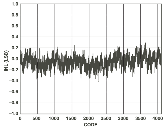
TPC 23. Typical INL
