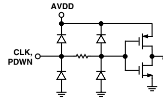
Figure 5. Equivalent Digital Input Circuit
