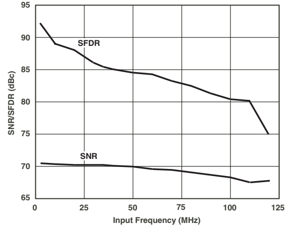
TPC 10. AD9235-65: SNR/SFDR vs. f_{IN}
